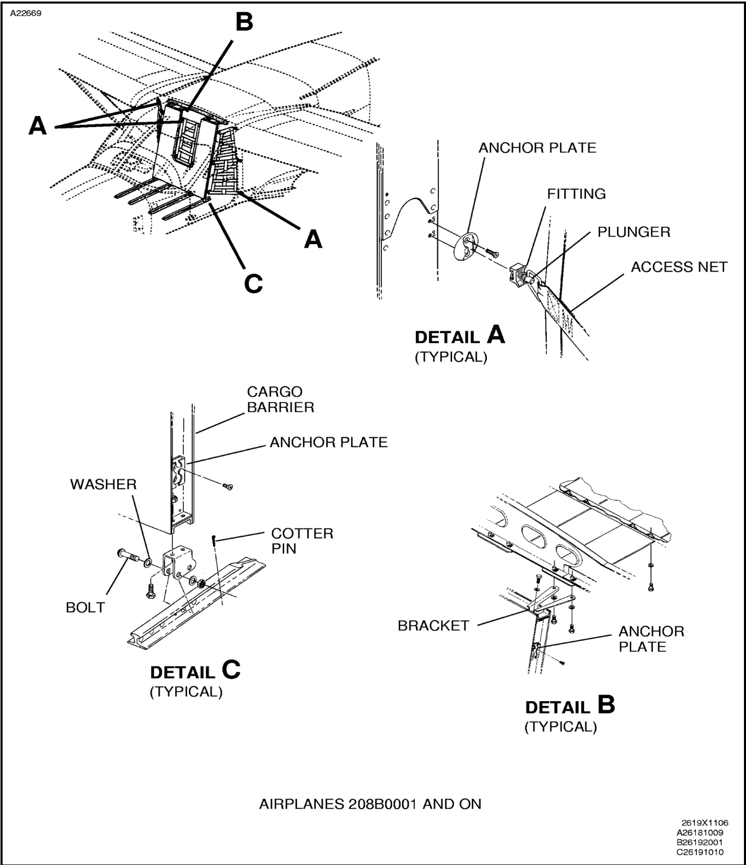
Figure 202 : Sheet 3 : Cargo Barrier and Access Nets Installation
