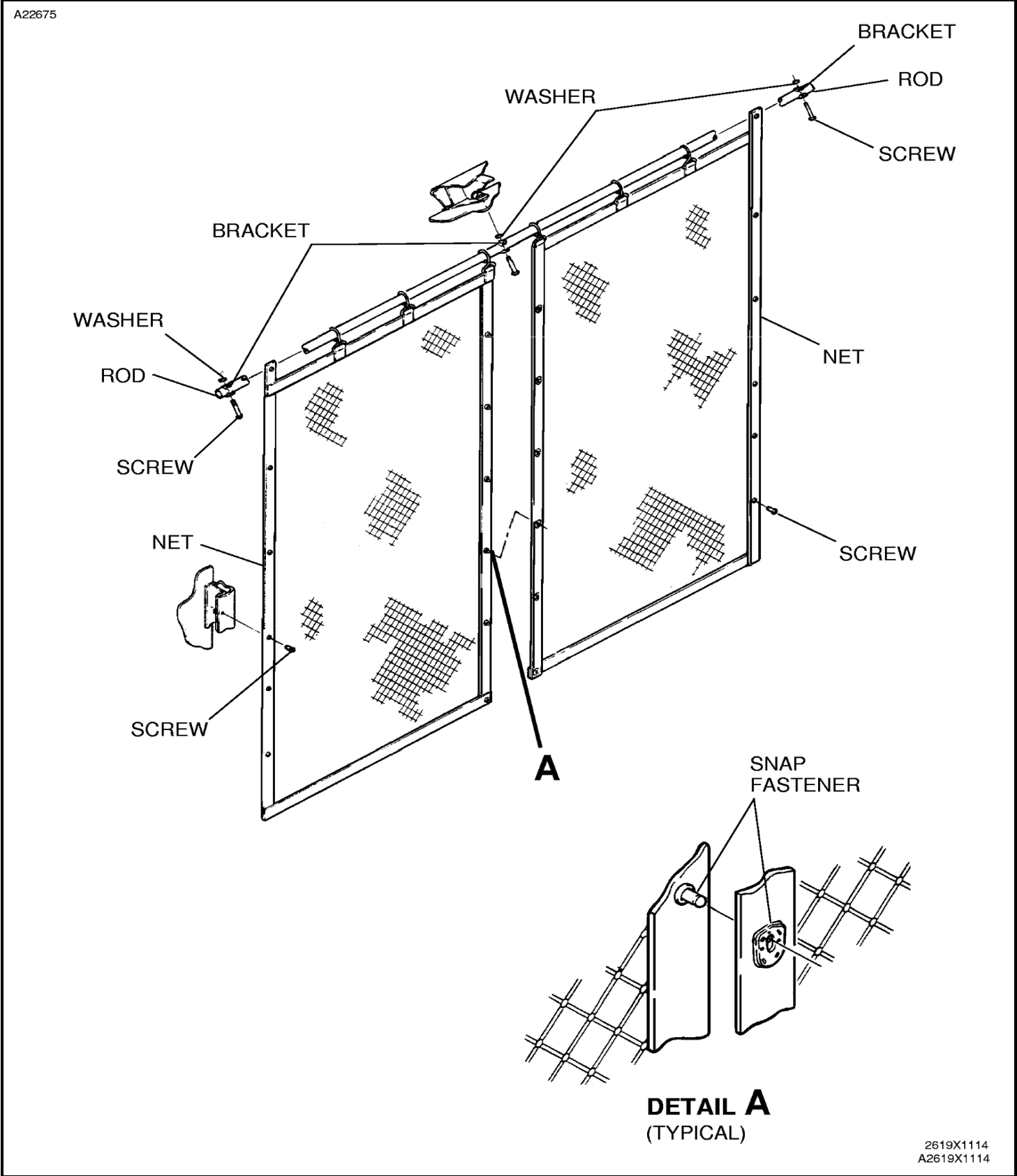
Figure 204 : Sheet 1 : Cargo Door Restraint Net Installation
