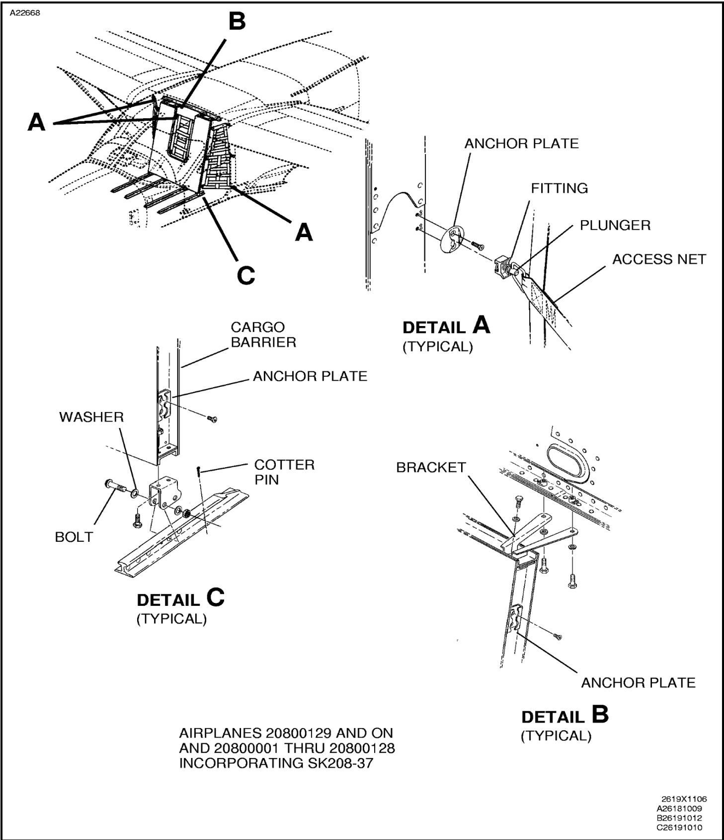
Figure 202 : Sheet 2 : Cargo Barrier and Access Nets Installation
