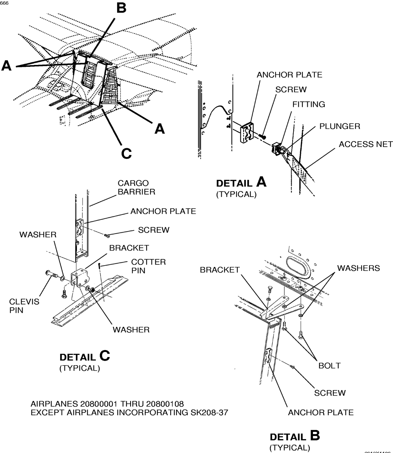
Figure 202 : Sheet 1 : Cargo Barrier and Access Nets Installation
